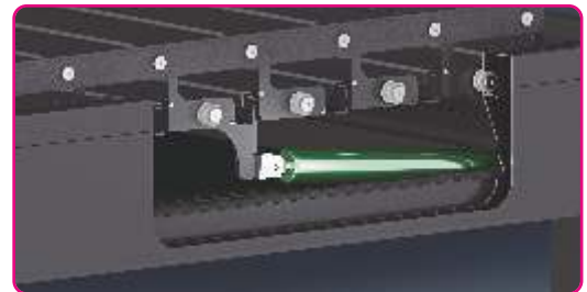
Professional advanced waterproof IP67 motor, 24V low voltage, more stable and safer
